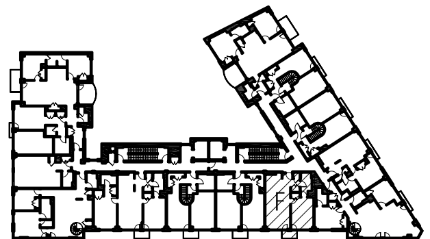
KEY PLAN
